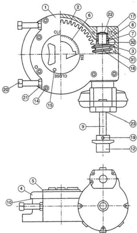
FIGURA 8. GEAR ACTUATOR CONSTRUCTION
