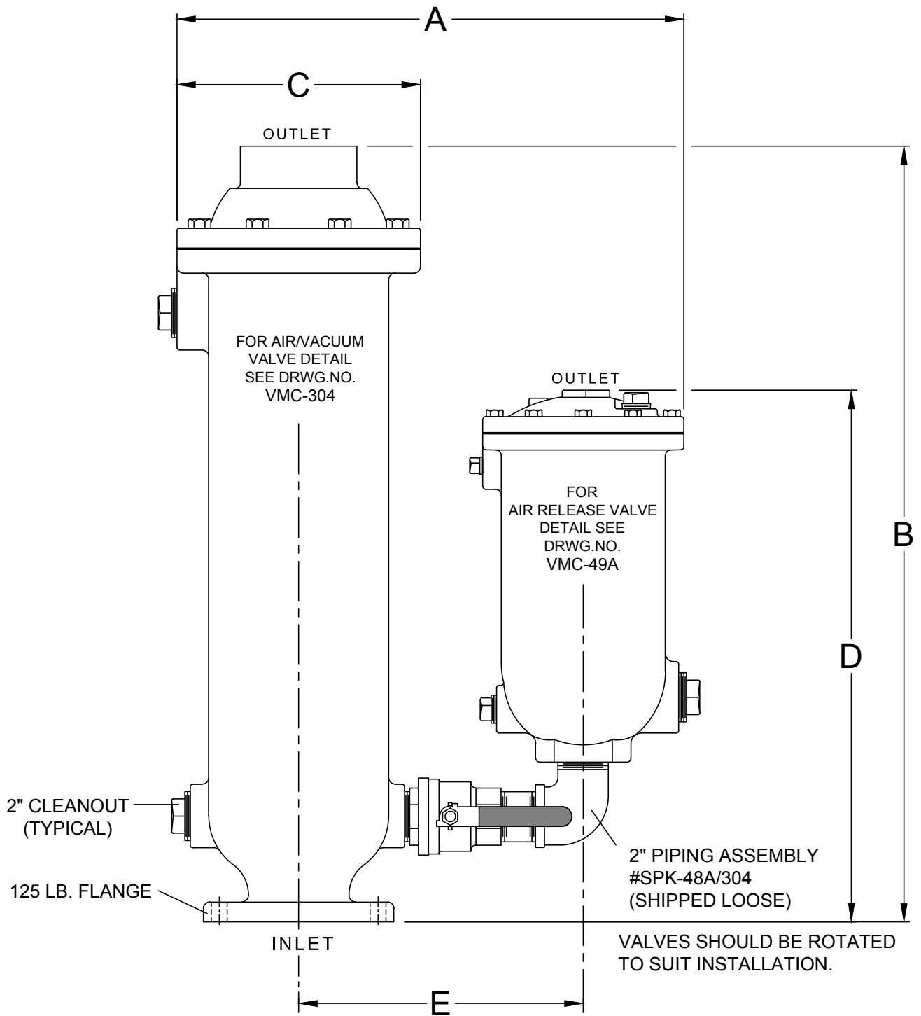
DRAWING DEPICTS 4" AIR/VACUUM VALVE SIZE TO SCALE
