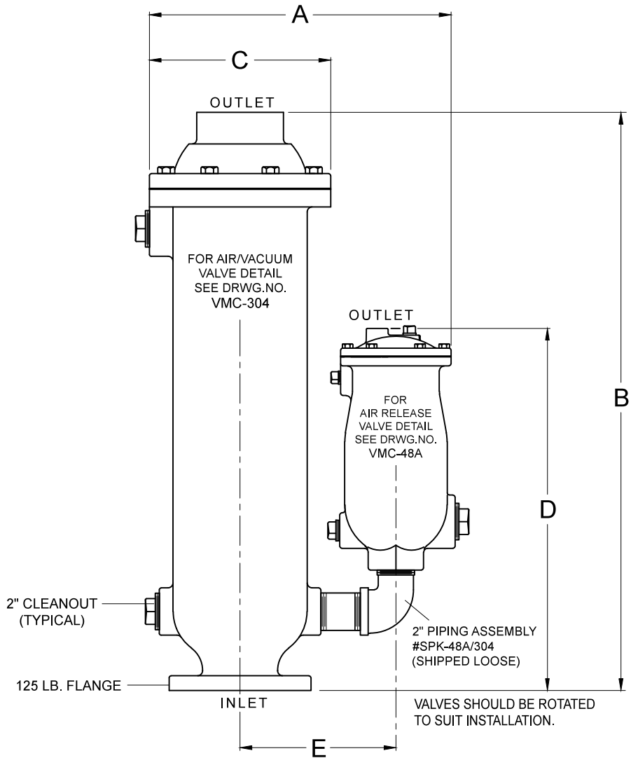
DRAWING DEPICTS 4" AIR/VACUUM VALVE SIZE TO SCALE
