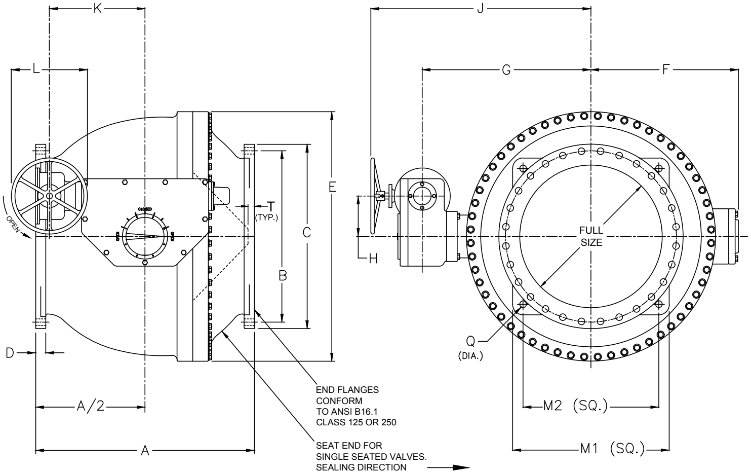
VALVE DEPICTS 30" 150 LB. SIZE WITH LS-5.2A ACTUATOR
