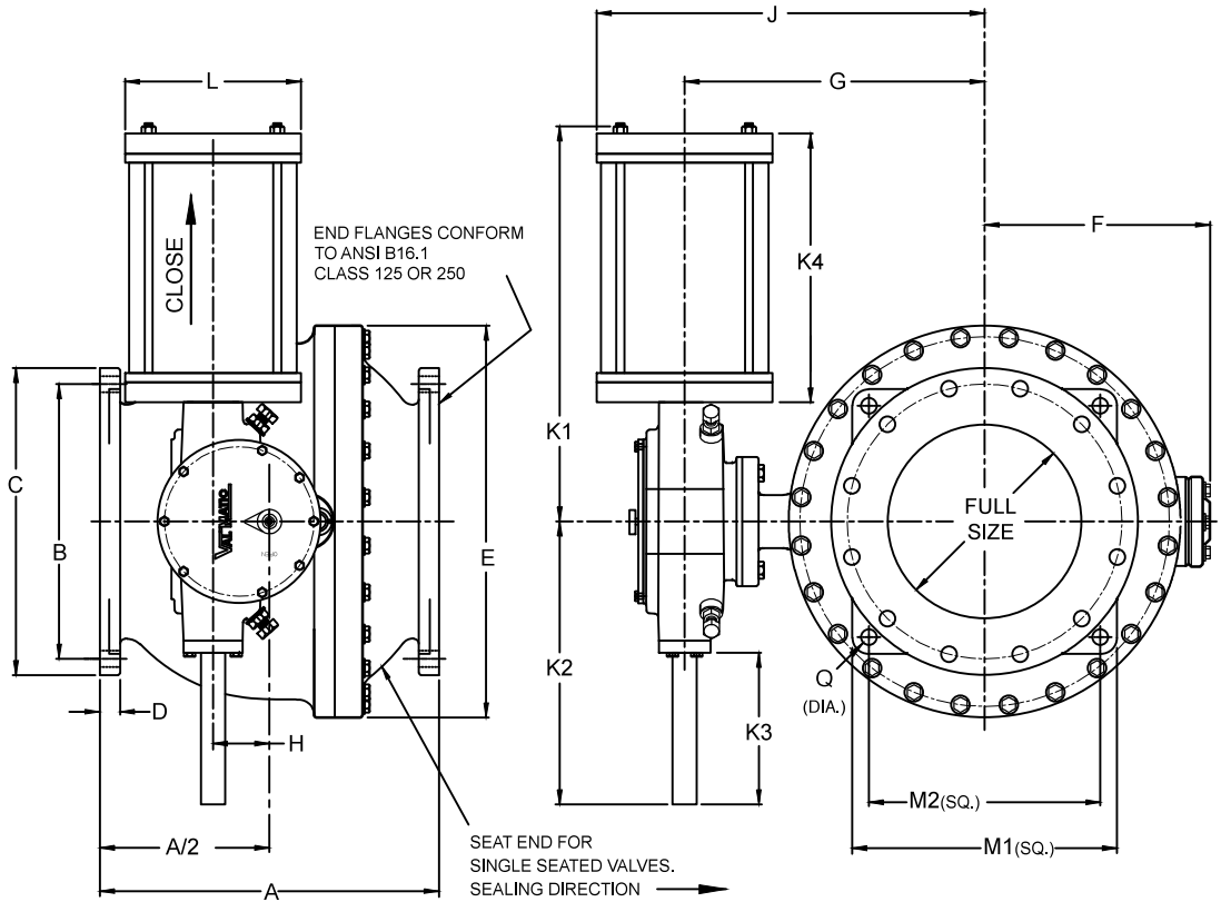
VALVE DEPICTS 12" 150 SIZE WITH LS-3A ACTUATOR
