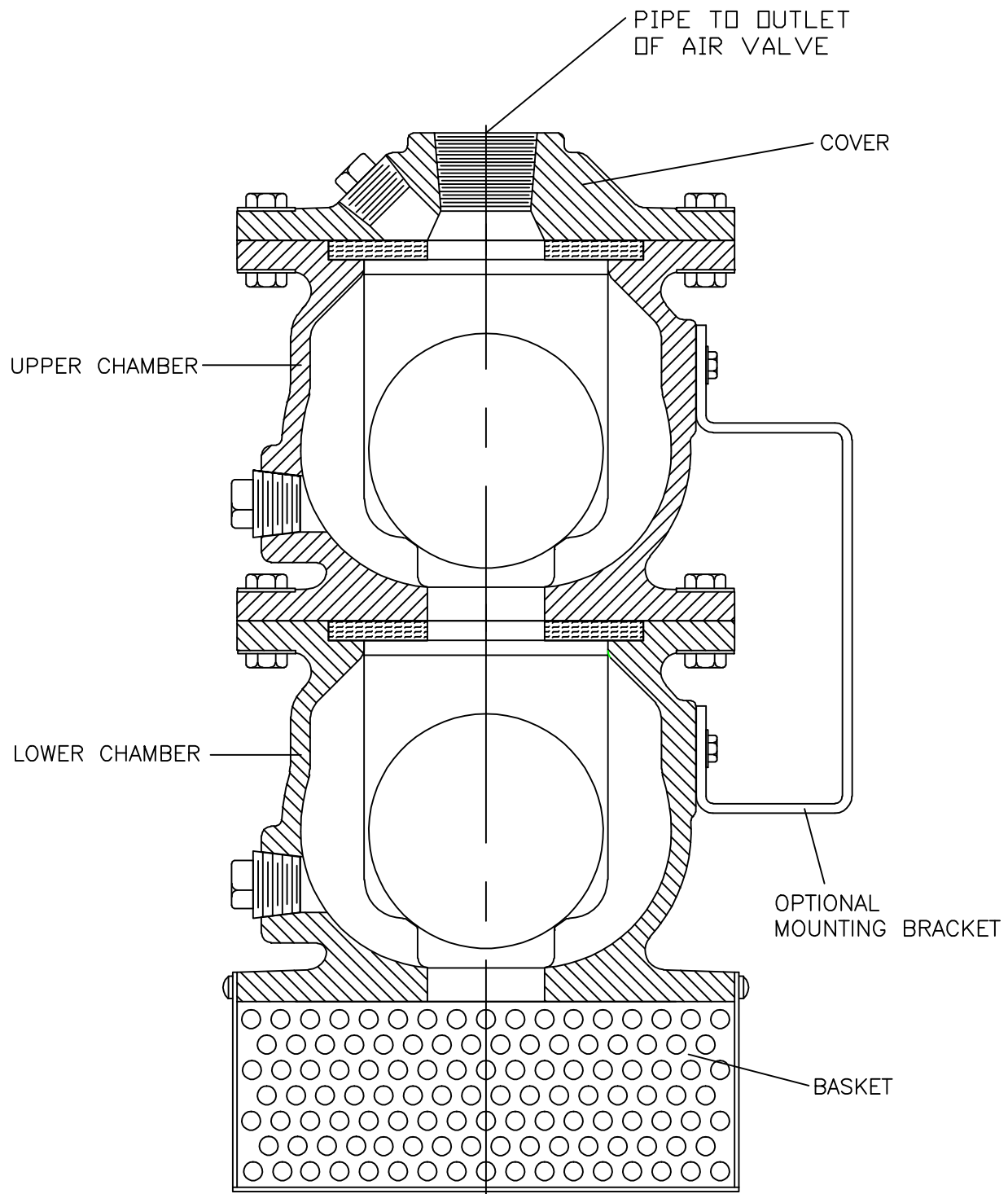
1"–12" FLOODSAFE® (NO SCALE)
