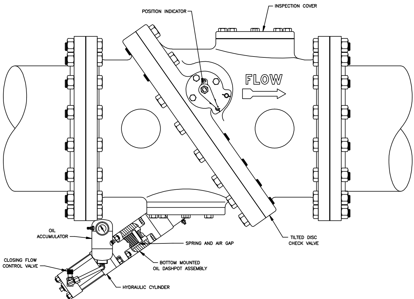
6"-54" TILTED DISC CHECK VALVE DETAIL WITH BOTTOM MOUNTED OIL DASHPOT
