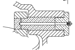
6" PIVOT PIN COVER DETAIL
