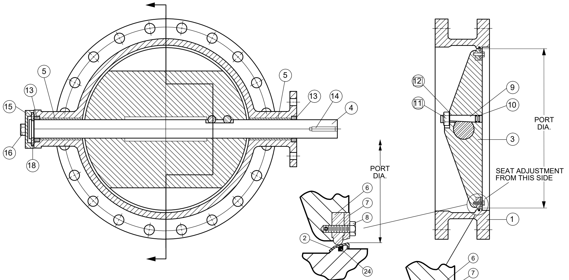
SST316 SEAT VIEW
