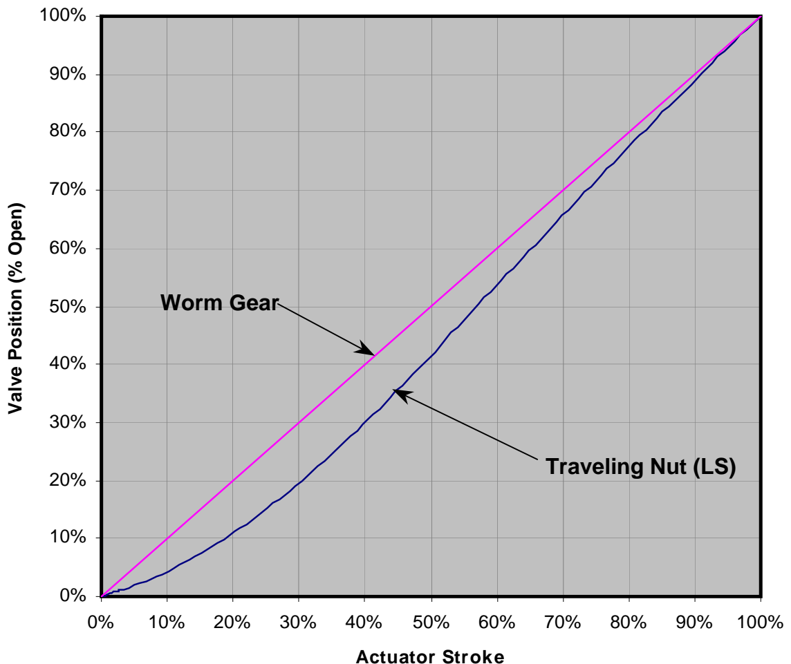
Traveling Nut vs. Worm Gear
