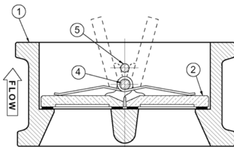
FIGURE 2. DUAL DISC® CHECK VALVE
