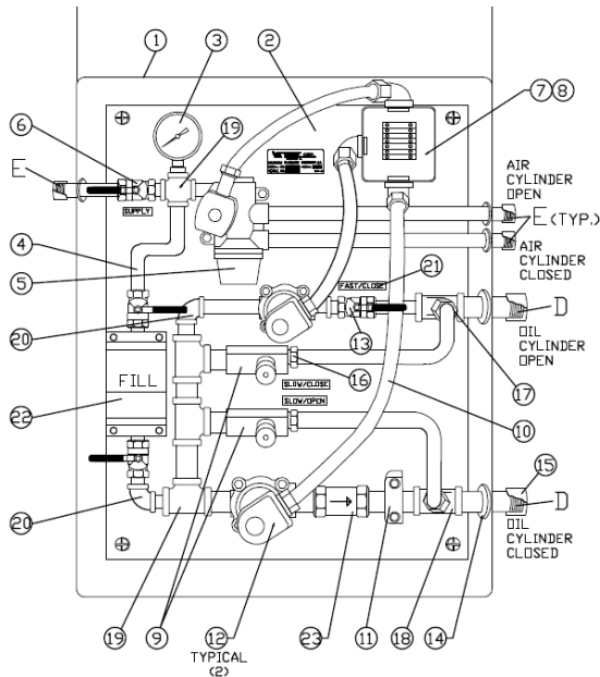
FIGURE 1. Air/Oil Hydraulic Panel
