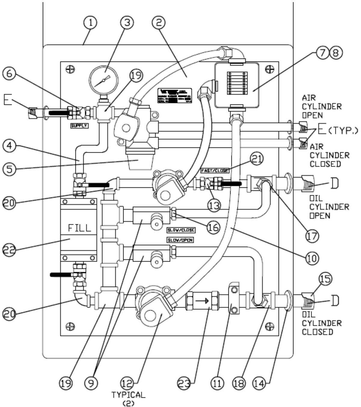
Figure 4. Air-Oil Hydraulic Panel Construction
