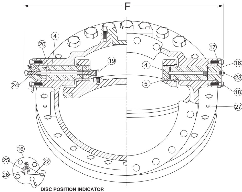
DISC POSITION INDICATOR
