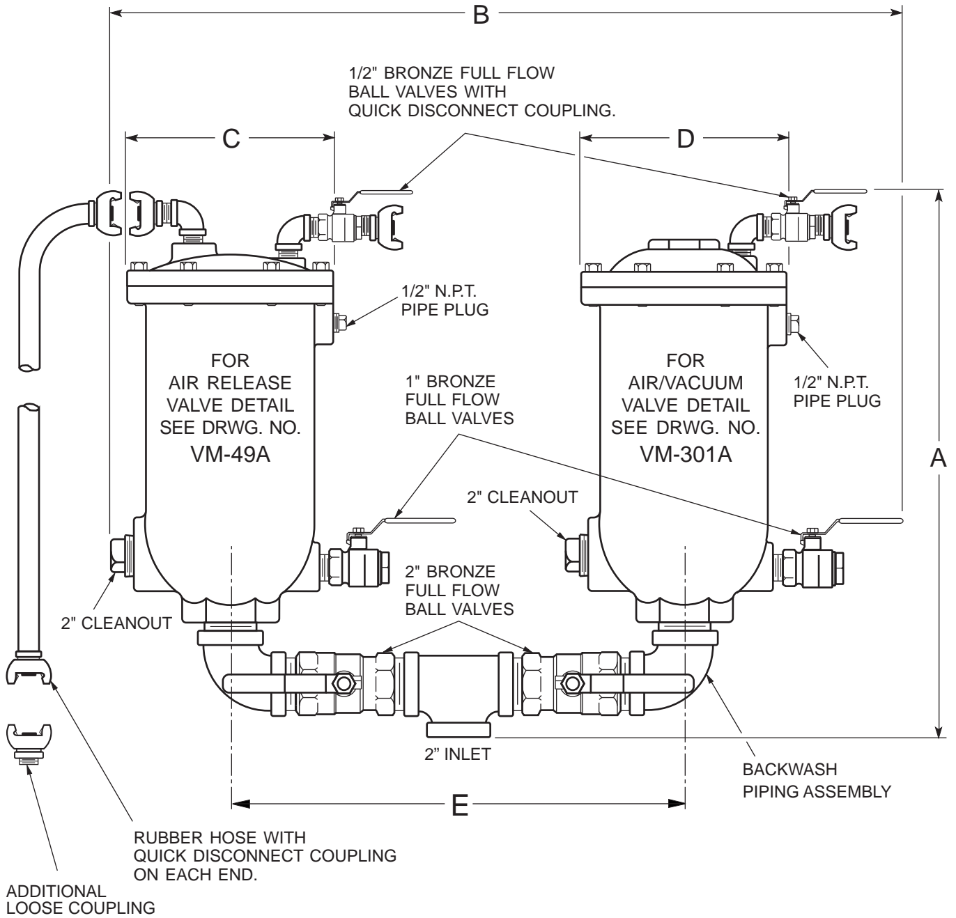
PIPING ASSEMBLY #SPK-48A/301ABW (SHIPPED LOOSE)
