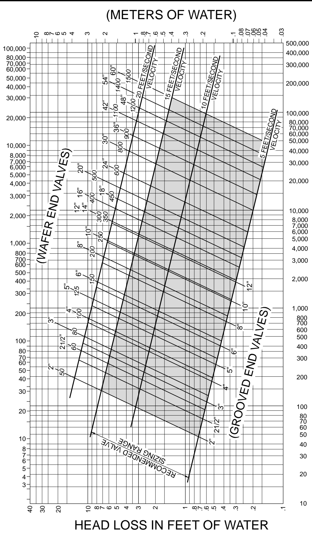
HEAD LOSS CHART FOR DUAL DISC CHECK VALVES
