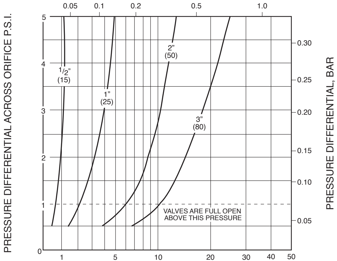
FLOW OF AIR THRU AN ORIFICE IN S.C.F.S. (STANDARD CUBIC FEET OF FREE AIR PER SECOND)
