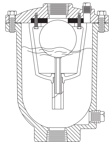
AIR/VACUUM VALVE
