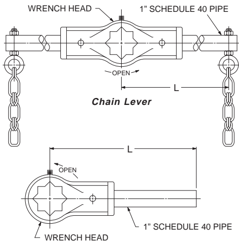
Hand Lever
