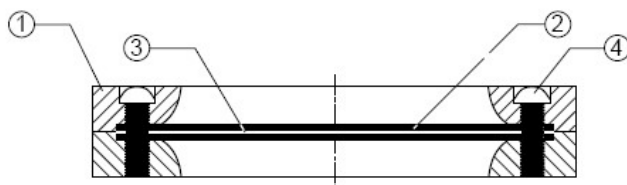
Figure 3: FrostSafe™ Cross Section of Components
